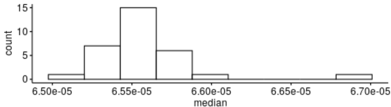
Density of median - SHA256D64_1024
