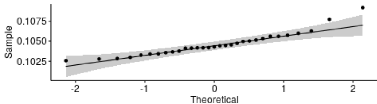
Q-Q plot for medians - RpcMempool10k
