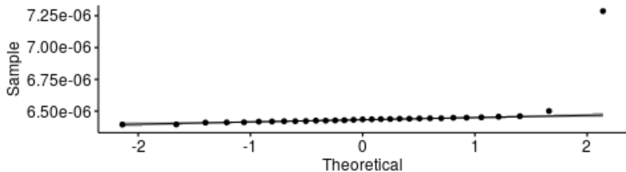
Q-Q plot for medians - AES128CBC_DecryptWithPad
