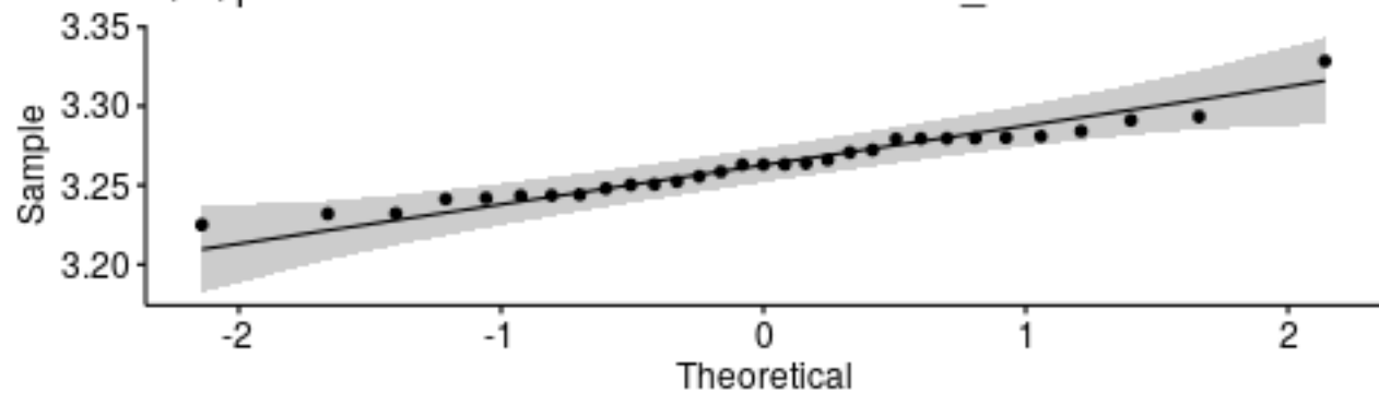
Q-Q plot for medians - BlockToJsonVerbose_32MB
