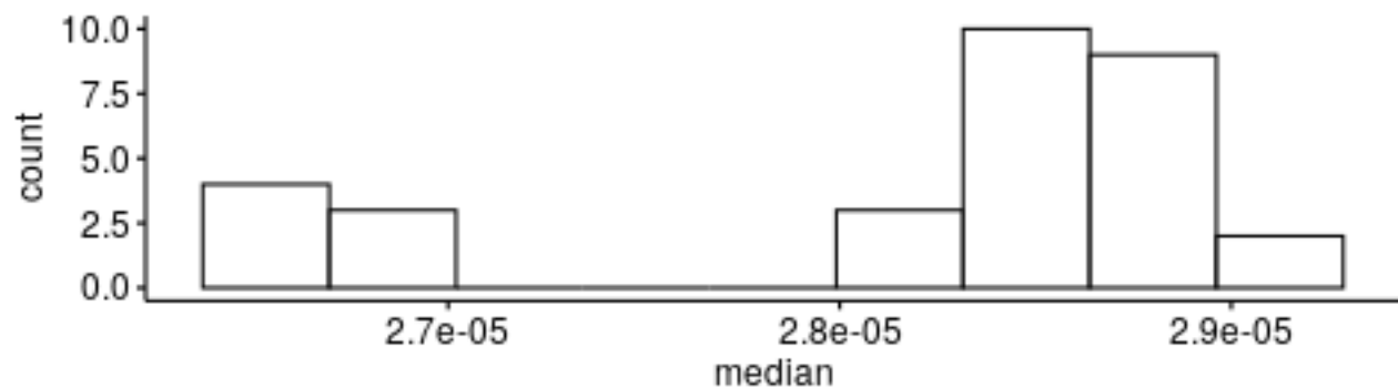
Density of median - PrevectorResizeNontrivial
