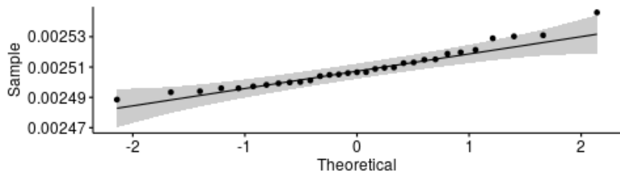
Q-Q plot for medians - SHA512
