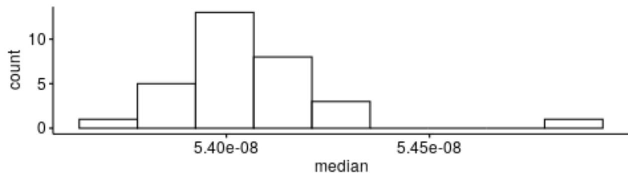
Density of median - SHA256_32b
