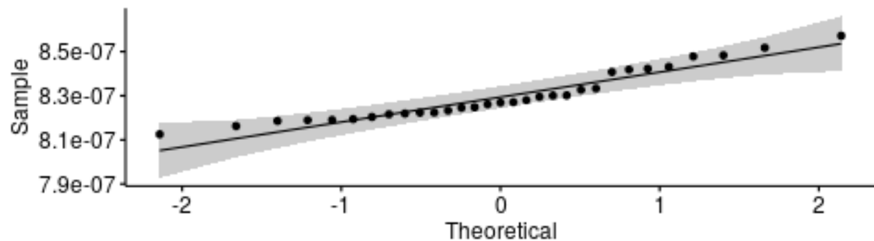
Q-Q plot for medians - CashAddrDecode
