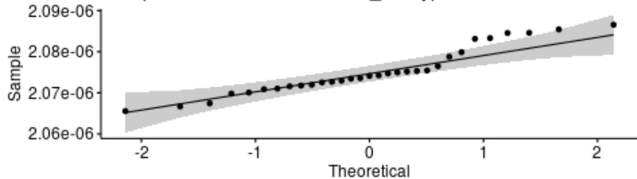
Q-Q plot for medians - AES256_Encrypt
