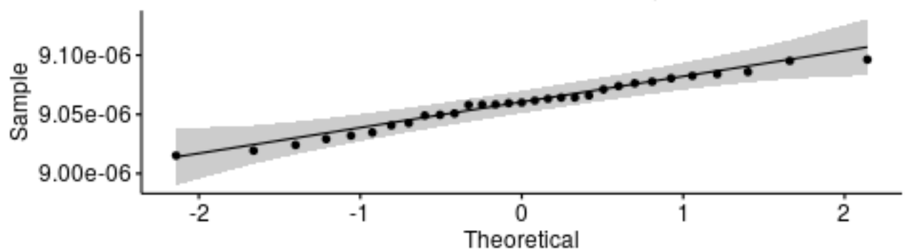
Q-Q plot for medians - AES256CBC_EncryptWithPad
