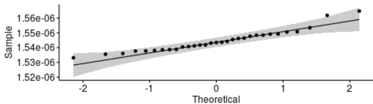
Q-Q plot for medians - Base58Encode
