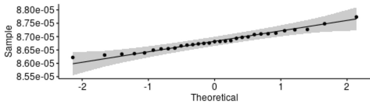
Q-Q plot for medians - PrevectorDeserializeNontrivial
