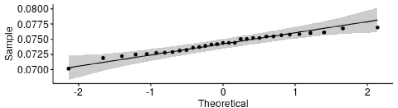
Q-Q plot for medians - BlockToJsonVerbose_1MB
