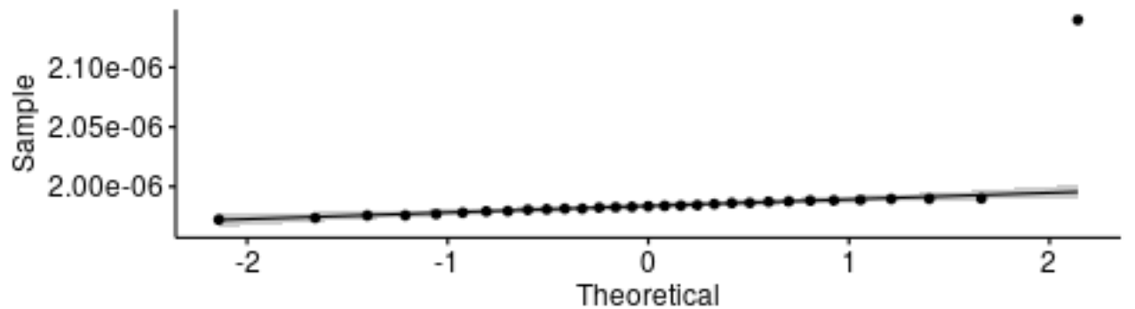
Q-Q plot for medians - AES256_Decrypt
