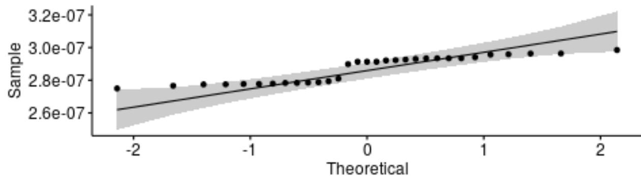
Q-Q plot for medians - BanManAddressBan
