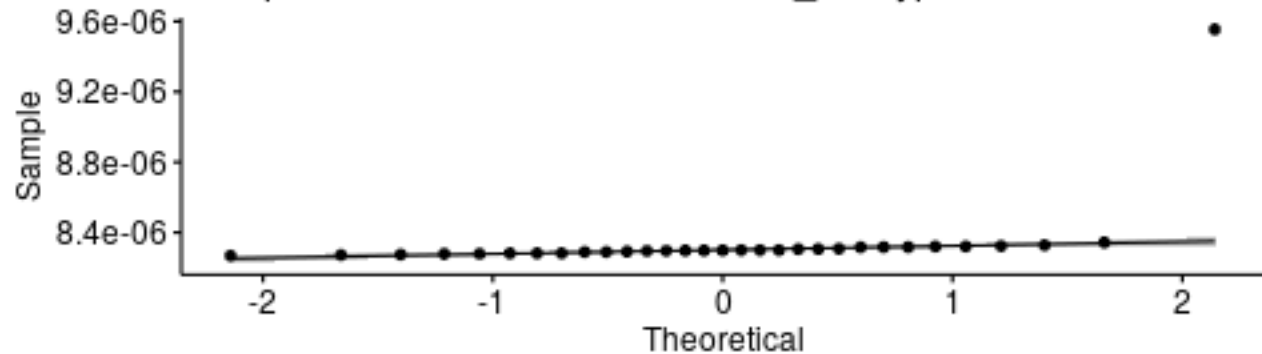
Q-Q plot for medians - AES256CBC_DecryptNoPad
