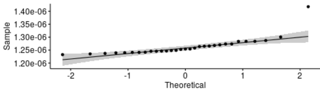
Q-Q plot for medians - CCoinsCaching
