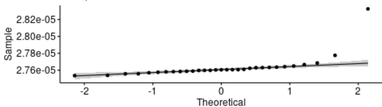
Q-Q plot for medians - PrevectorClearTrivial
