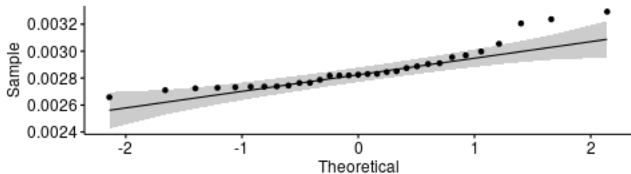
Q-Q plot for medians - BanManAddressIsBanned
