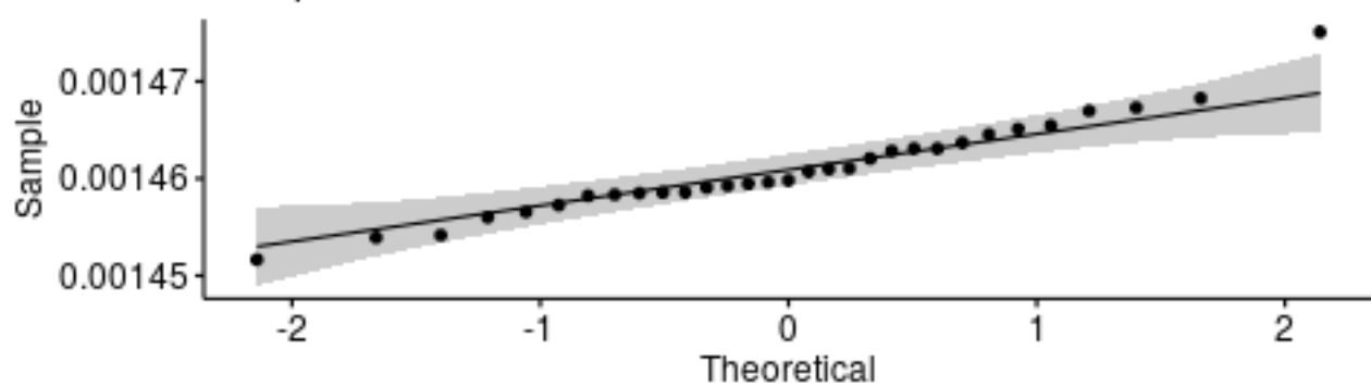
Q-Q plot for medians - SHA1
