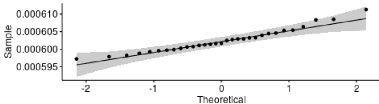
Q-Q plot for medians - MerkleRoot
