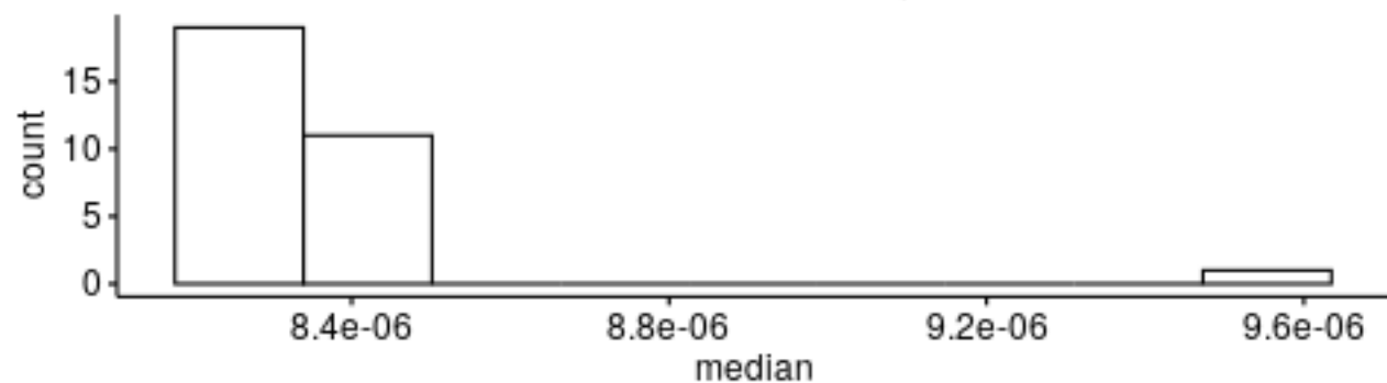
Density of median - AES256CBC_DecryptWithPad
