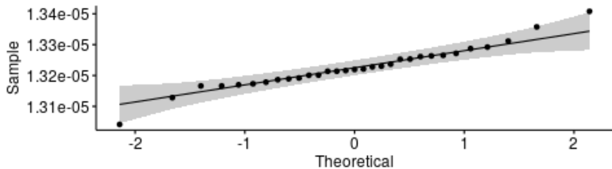
Q-Q plot for medians - PrevectorDeserializeTrivial
