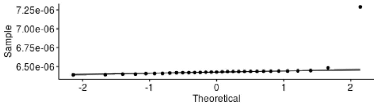
Q-Q plot for medians - AES128CBC_DecryptNoPad
