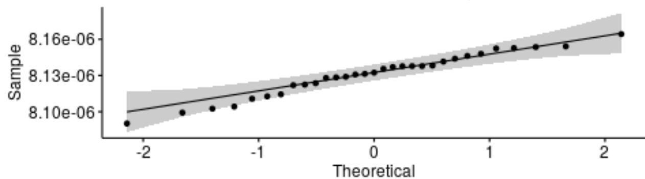
Q-Q plot for medians - AES256CBC_EncryptNoPad
