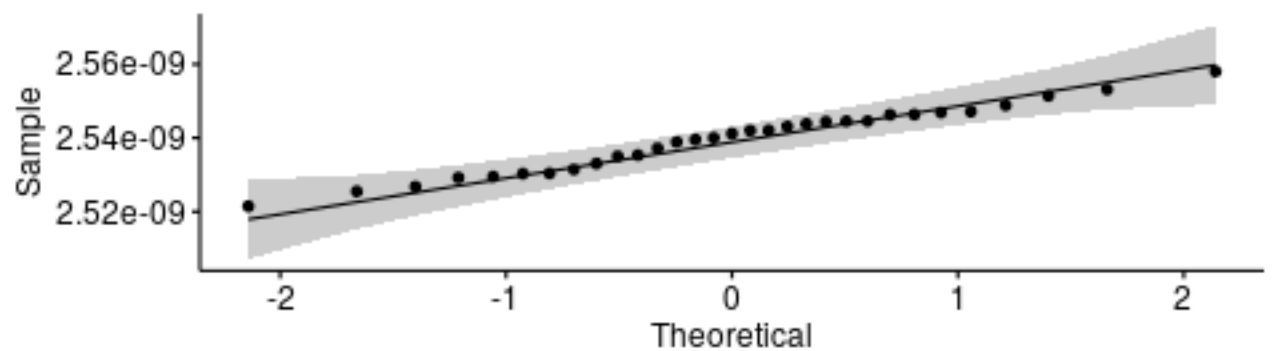
Q-Q plot for medians - FastRandom_1bit
