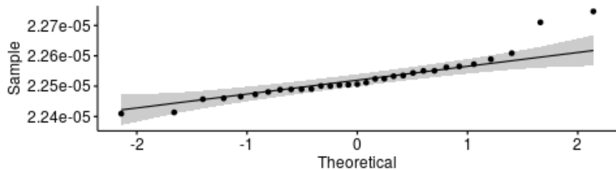
Q-Q plot for medians - MatchGCSFilter
