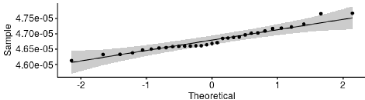
Q-Q plot for medians - PrevectorDestructorNontrivial
