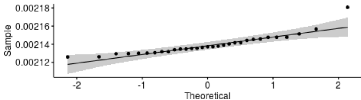
Q-Q plot for medians - RIPEMD160
