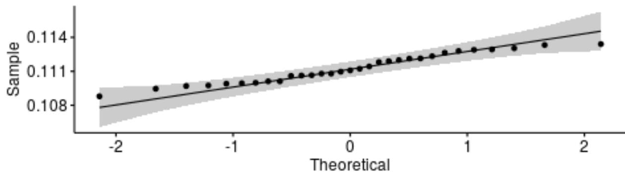
Q-Q plot for medians - DeserializeBlockTest_32MB
