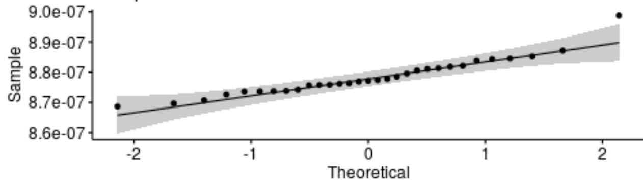
Q-Q plot for medians - Base58Decode
