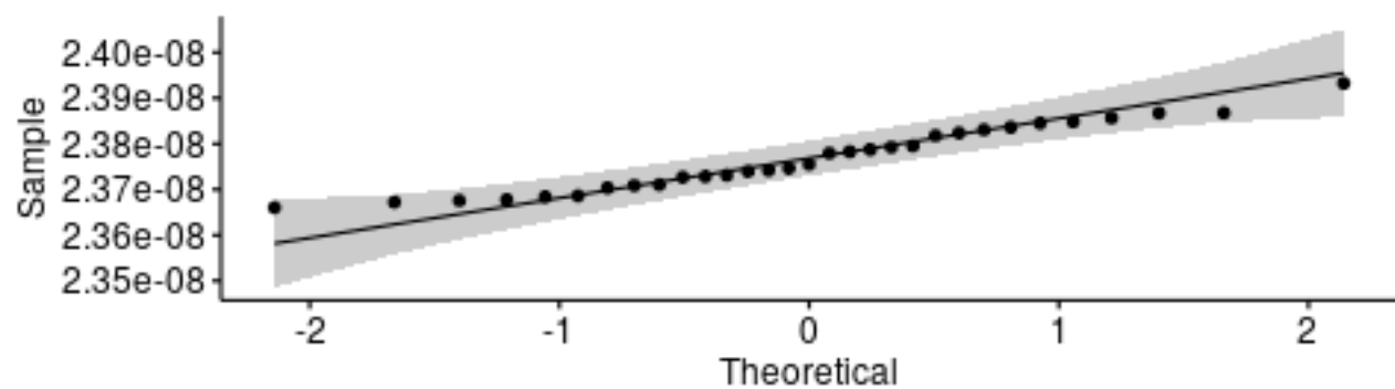
Q-Q plot for medians - SipHash_32b
